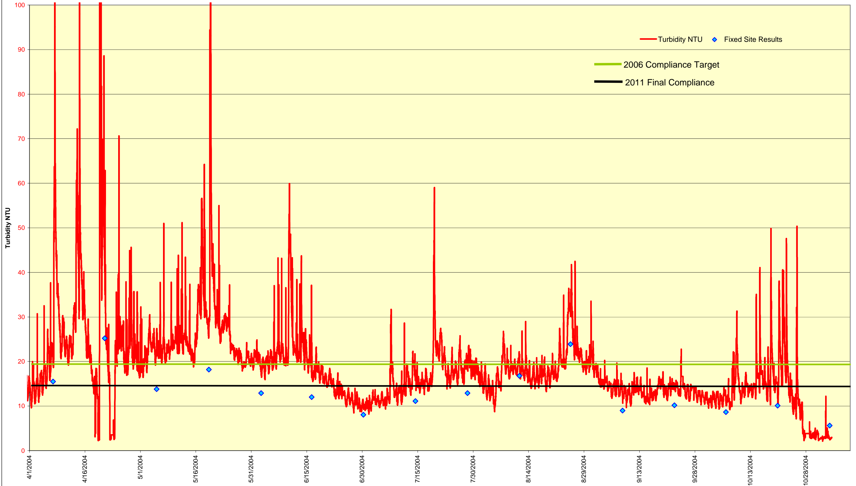
Wilson at Canyon Rd Turbidity Levels
